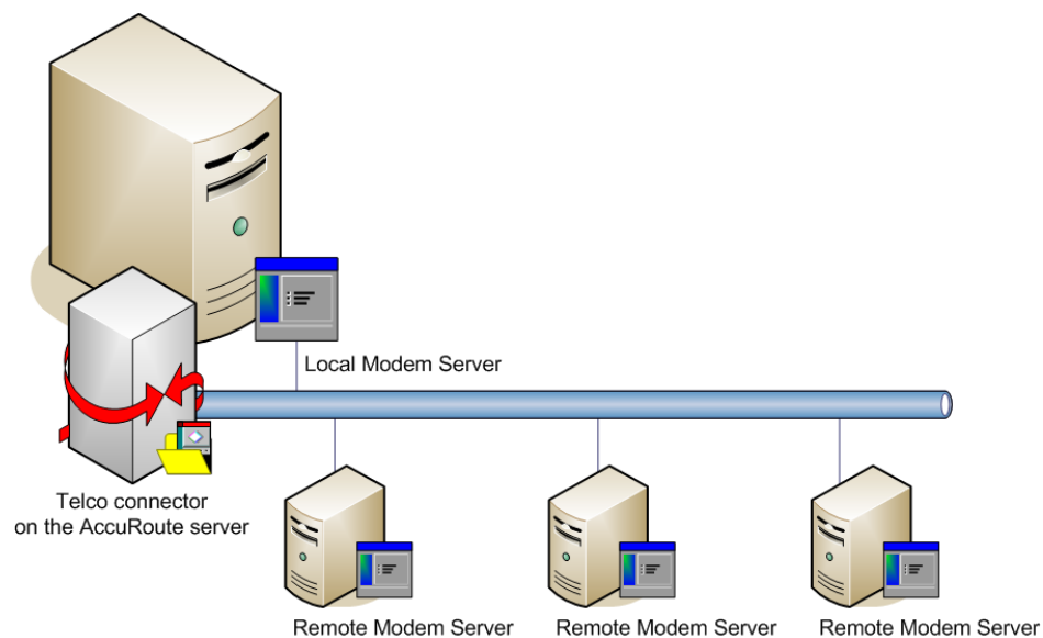
Figure 11-1: AccuRoute server with local Modem Server and Remote Modem Servers
